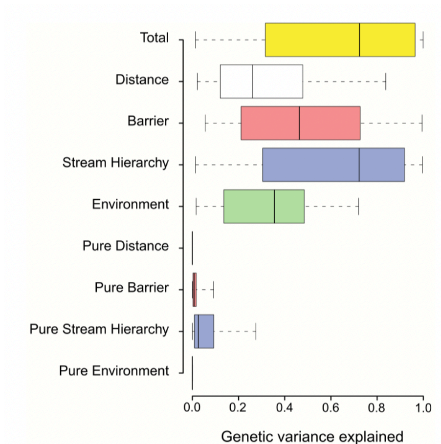
FIGURE 7 Neutral genetic variation was partitioned between four explanatory models for N = 31 fish species sampled across the White River Basin (Ozark Mountains, USA). Partitioning was conducted separately for each species. The four models represent: (i) isolation by distance, the river network distance among individuals represented by spatial eigenvectors; (ii) isolation by barrier, represented by population structure coefficients among individuals; (iii) isolation by stream hierarchy, based on the hydrologic units (at four different hierarchical levels) in which an individual was collected; and (iv) isolation by environment, characterized by the environmental heterogeneity across sampling sites where individuals were collected. Total = the genetic variation explained by all four models combined. The “Pure” models represent the variation explained by each model after partialling out the variation explained by the other three models
