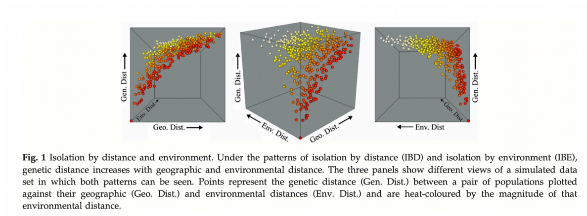
Figure 2: IBE signals - Wang & Bradburd 2014
