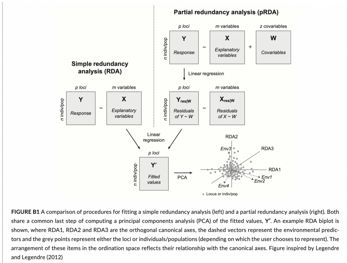
Figure 5: Conceptual overview of RDA - From Capblancq et al. 2021
